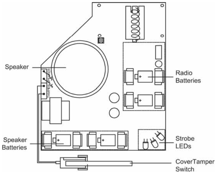
Figure 4-1: Siren Strobe – PCB Diagram
