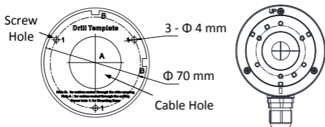
Figure 2-4 The Drill Template
