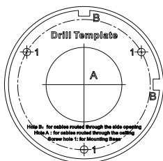
Figure 2-19 Drill Template
