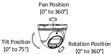
Figure 2-18 3-Axis Adjustment
