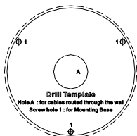
Figure 2-33 Drill Template
