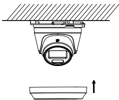
Figure 2-31 Install the Trim Ring Back
