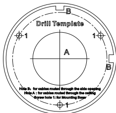
Figure 2-7 Drill Template for Junction Box
