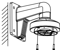
Figure 2-12 Fix the Mounting Base onto the Wall Mount
