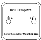
Figure 2-3 Drill Template
